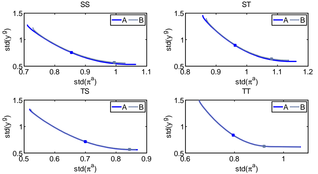
Figure 6: Robustness of the interest rate rule.
