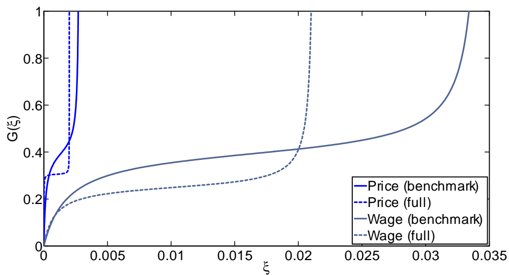
Figure 1: Distributions of price-setting and wage-setting costs.
