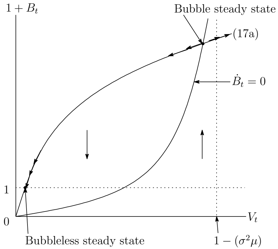
Figure 3 Phase Diagram
